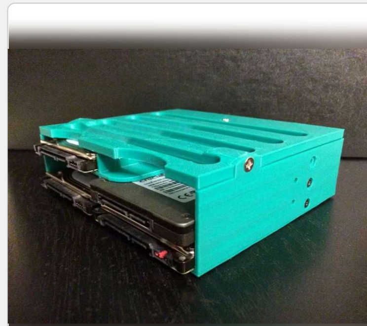
6 x 2.5 Drive to one 5.25 Optical Drive Bay Adapter.
